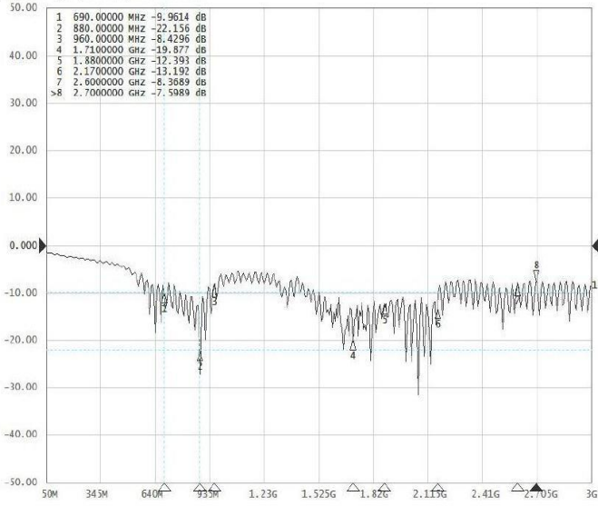
172 S11 Log Mag 10.00ds/ Ref 0.000ds
