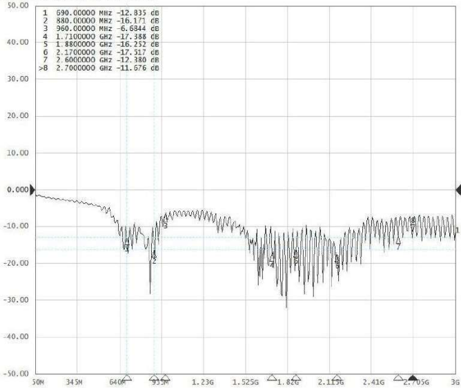
174 S11 Log Mag 10.00ds/ Ref 0.000de
