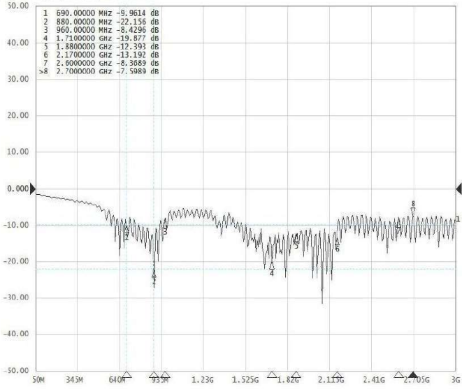
172 S11 Log Mag 10.00ds/ Ref 0.000de
