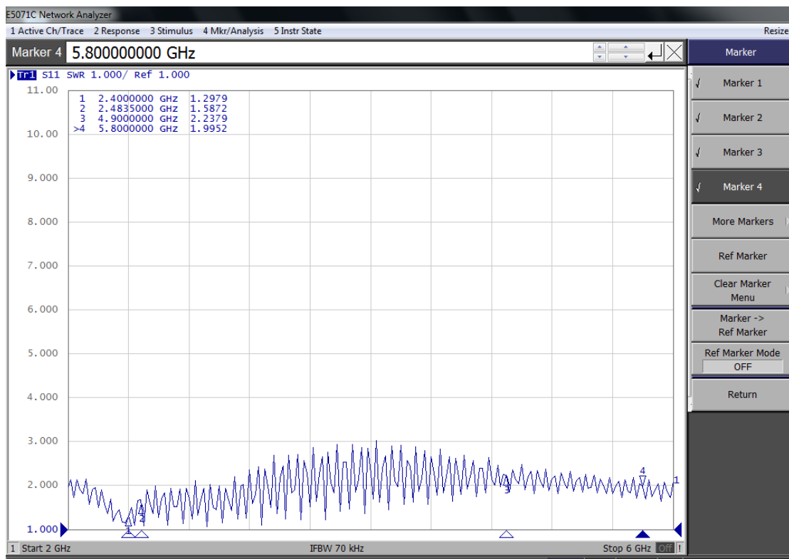
Graph – VSWR
