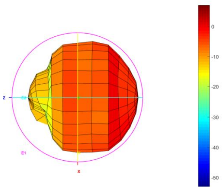
Total_3D_Top View_1.9GHz
