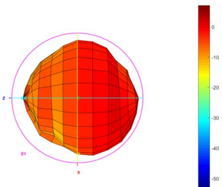
Total_3D_Top View_2.1GHz
