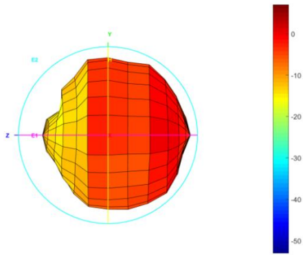
Total_3D_Left View_1.8GHz
