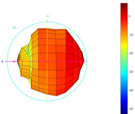
Total_3D_Left View_1.9GHz
