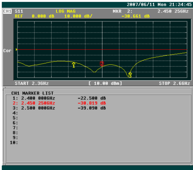
Return loss
