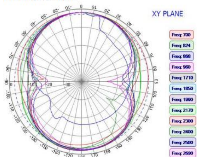
LTE Antenna MAIN
