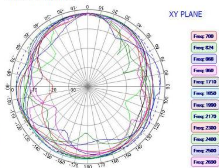
LTE Antenna AUX
