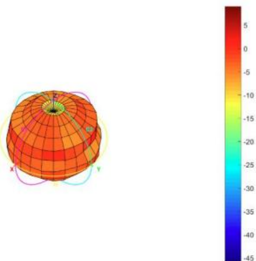
Total_3D_Side View_1.9GHz
