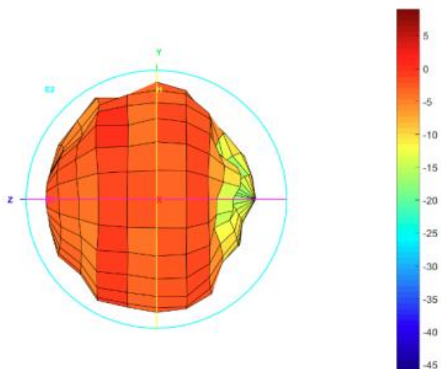
Total_3D_Left View_1.9GHz
