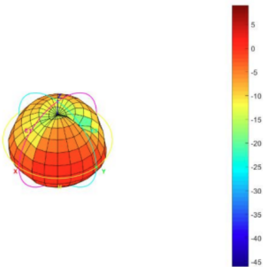
Total_3D_Side View 1_900MHz
