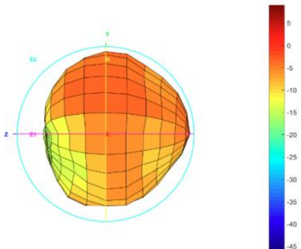
Total_3D_Left View_850MHz
