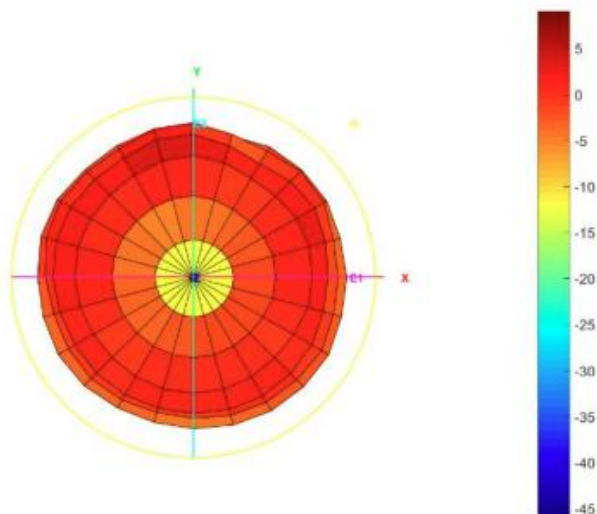
Total_3D_Front View_2.1GHz
