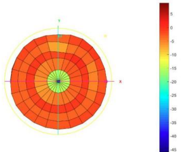
Total_3D_Side View 1_1.8GHz
