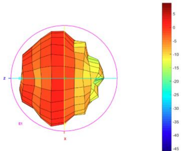
Total_3D_Left View_1.8GHz
