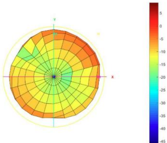
Total_3D_Side View 1_850MHz
