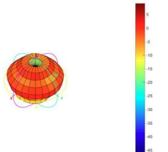
Total_3D_Side View 1_1.8GHz
