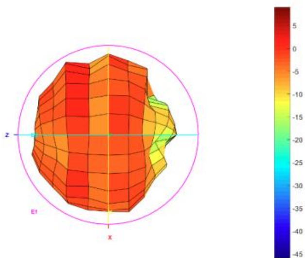
Total_3D_Left View_1.9GHz
